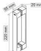
Tirador Acero REF: 024401 44 € REF: 024402 48 €
