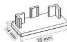
Tapa perfil pared ABS REF: 004901 10 €
