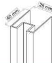
Perfil expansor a cristal Acero REF: 002701 55 €
