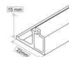
Junquillo 100F Acero REF: 041101 24 € REF: 041102 24 €
