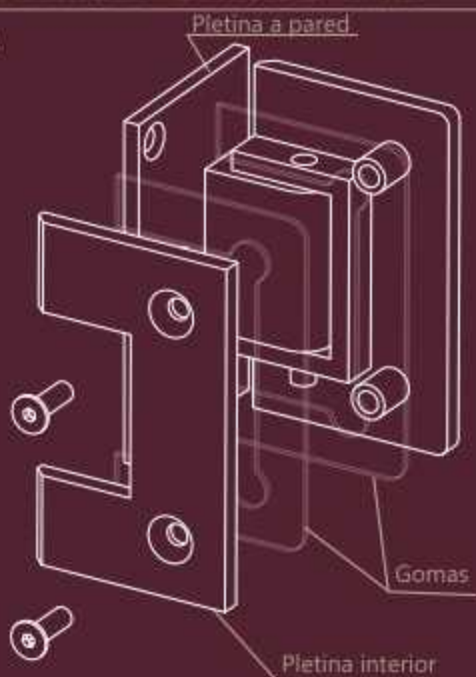
Bisagra A
