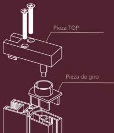
Conector angular
