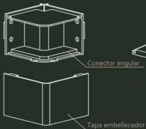
Conector angular
