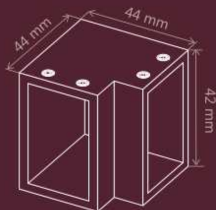
Conector angular
