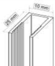
Perfil U 2,5 cm Aluminio REF: 003001 35 € REF: 003002 40 €
