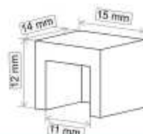
Embellecedor junquillo REF. 040201 10 € REF. 040202 Acero 10 € REF. 040203 10 € REF. 040204 10 € REF. 040205 10 € REF. 040206 10 €
