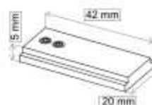
Tapa conectores Aluminio REF: 013101 10 €
