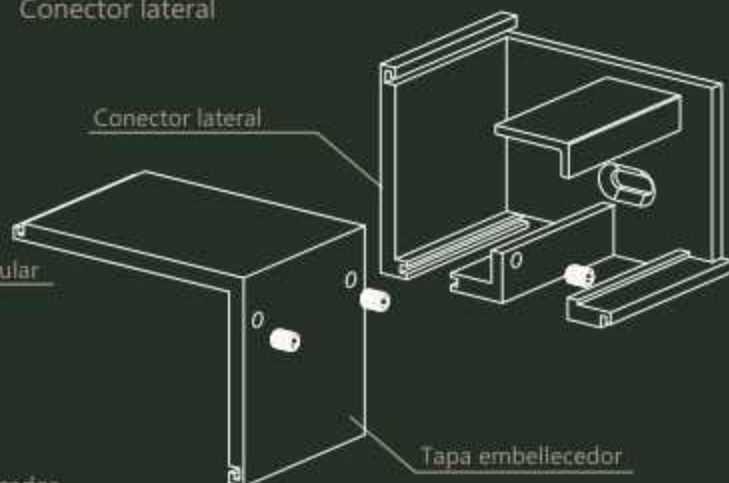
Conector lateral
