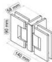
Bisagra triple Z Acero REF: 028501 85 € REF: 028502 90 €
