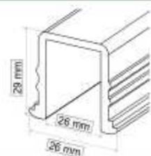
Goma cristal fijo Goma REF: 033000 11 € REF: 033002 11 €
