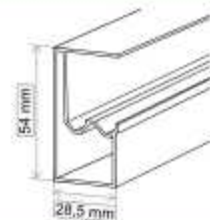
Perfil superior Aluminio REF: 017501 61 € REF: 017502 70 €
