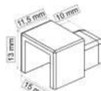
Embellecedor junquillo ABS REF: 040301 10 € REF: 040302 10 €
