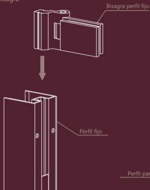
Bisagra
