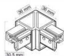
Conector angular ABS REF: 019801 20 € REF: 019802 20 €
