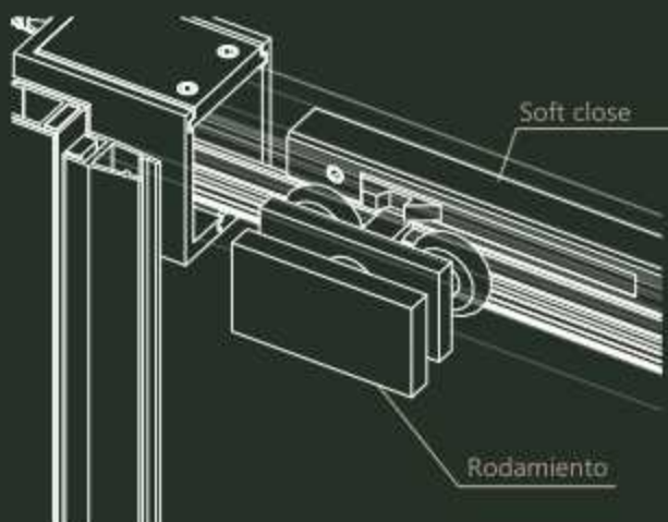
Soft close
