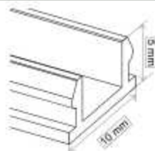
Perfil clipado Aluminio REF: 020901 20 € REF: 020902 20 €
