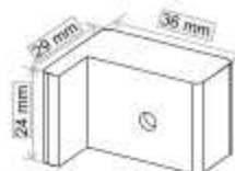
Conector 400 - 2
