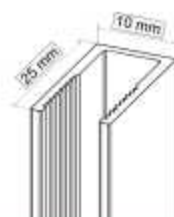
Perfil pared 2,5 cm Aluminio REF: 003001 35 € REF: 003002 40 €
