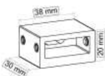
Conector pared
